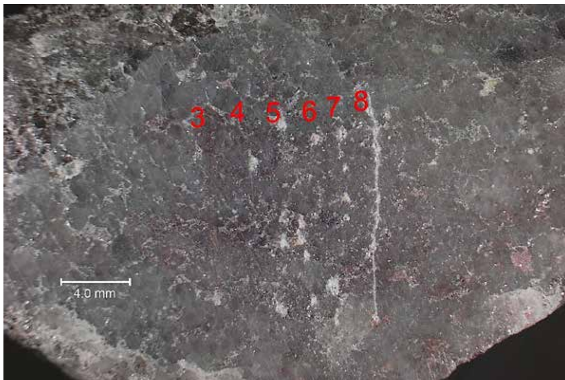
SAMPLE ID: #21 Sterling Quartz MAG: 5x DESCRIPTION: View of the lapped cross section of the stone after Mohs hardness testing. Note that hardness picks 3 did not scratch, hardness picks 4 thru 7 scratched a few minerals, and hardness pick 8 scratched all minerals. The general Mohs hardness would be approximately 6.5 to 7.
