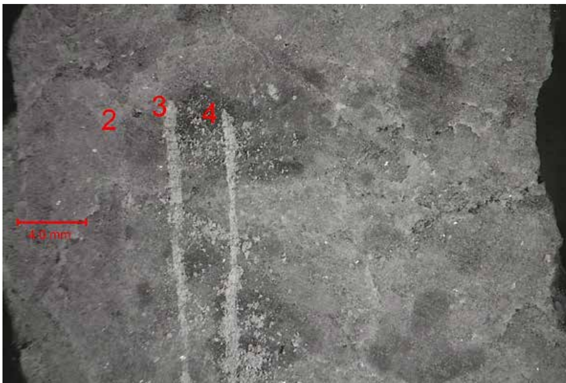
SAMPLE ID: #10 Misty Grey Marble MAG: 5x DESCRIPTION: View of the lapped cross section of the stone after Mohs hardness testing. Note that hardness pick 2 did not scratch, hardness pick 3 scratched several minerals, and hardness pick 4 scratched all minerals. The general Mohs hardness would be approximately 2.5 to 3.
