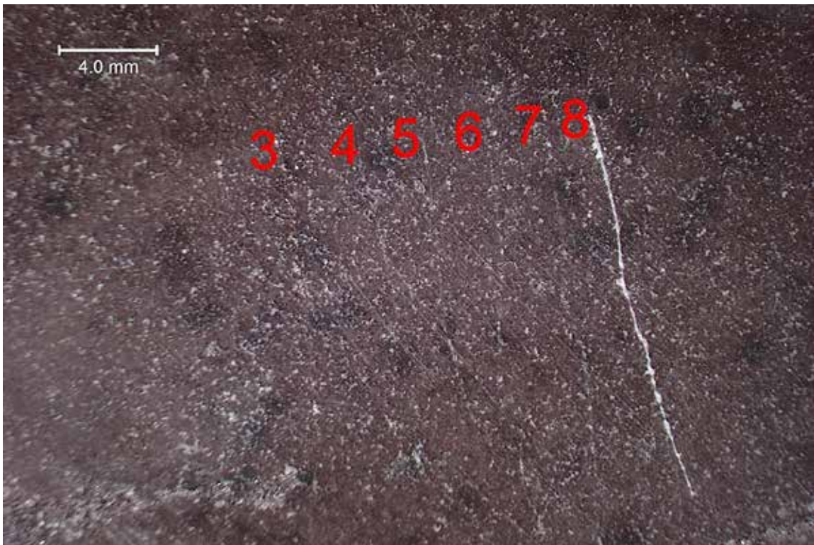
SAMPLE ID: Violetta Quartzite MAG: 5x DESCRIPTION: View of the lapped cross section of the stone after Mohs hardness testing. Note that hardness picks 3 through 7 did not scratch and hardness pick 8 scratched all minerals. The general Mohs hardness would be approximately 7.5.
