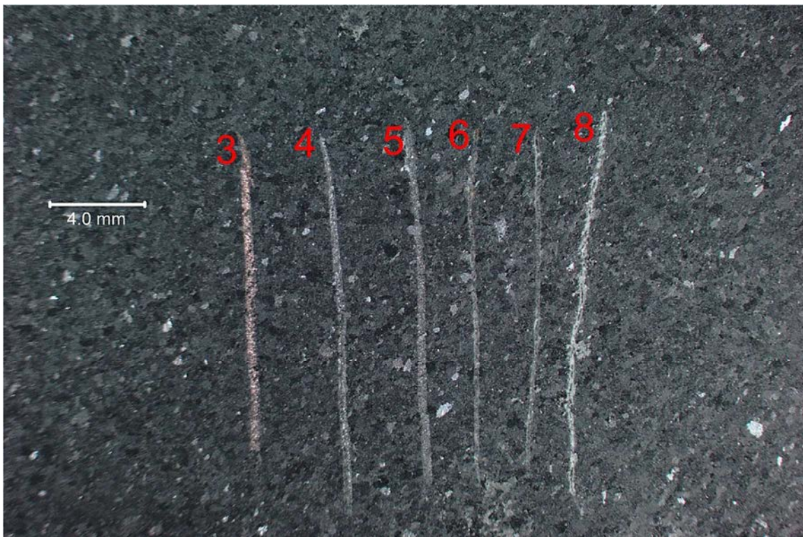
SAMPLE ID: Twilight Black Granite MAG: 5x
