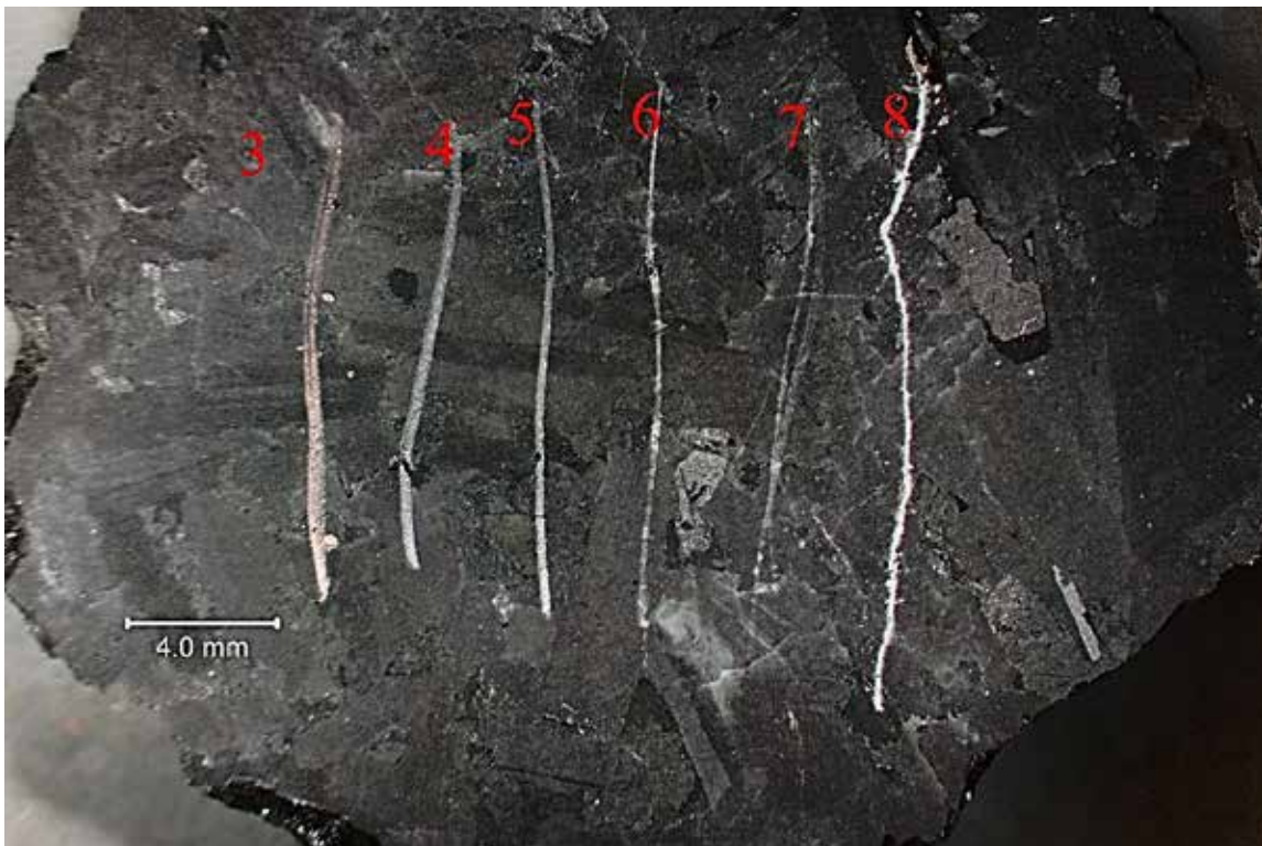
SAMPLE ID: Sample #6-Starlight Black 3/8x1/8 MAG: 5x DESCRIPTION: View of the lapped cross section of the stone after Mohs hardness testing. Note that hardness picks 3, 4, 5, and 6 did not scratch, hardness pick 7 scratched a few minerals, and hardness pick 8 scratched all minerals. The general Mohs hardness would be approximately 7.
