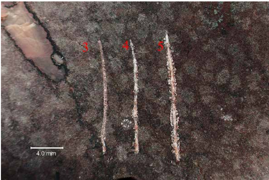
SAMPLE ID: Sample #5-Chocolate Brown 3/8x1/8 MAG: 5x DESCRIPTION: View of the lapped cross section of the stone after Mohs hardness testing. Note that hardness pick 3 did not scratch, hardness pick 4 scratched most minerals, and hardness pick 5 scratched all minerals. The general Mohs hardness would be approximately 3 to 4.
